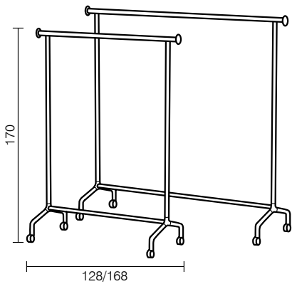
1640. NOX VESTA APPENDIABITI A BARRA SU RUOTE NON ACCESSORIATO COAT RAIL ON CASTORS WITH NO RACKS 1640.12 128 x 53 x h 170 cm 50.5" x 20.75 x h 67" 1640.16 168 x 53 x h 170 cm 66.25" x 20.75 x h 67"
