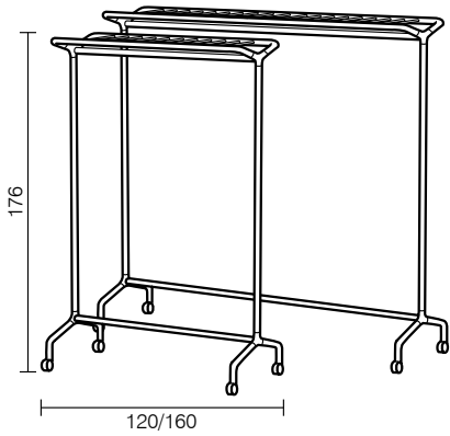
1641. NOX VESTA APPENDIABITI A BARRA SU RUOTE CON CAPPELLIERA COAT RAIL ON CASTORS WITH HAT RACK 1641.12 120 x 53 x h 176 cm 47.25" x 20.75 x h 69.25" 1641.16 160 x 53 x h 176 cm 63" x 20.75 x h 69.25"
