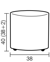
1681. NOX FLORA FIORIERA SU RUOTE PLANTER ON CASTORS Ø 38 x h 40 cm (38+2 cm) - 4,3 Kg dia. 15" x h 15.75" (15"+0.75") - 4,3 Kg sottovaso interno Ø 35 cm internal saucer dia. 13.75"
