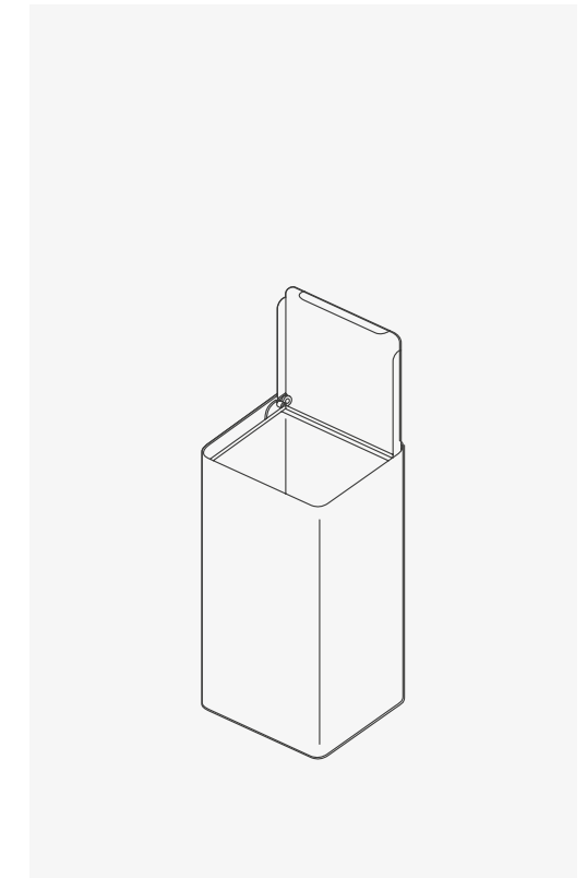
UNIX 40 cod. 1320-1321 25 x 25 – H 65 cm / 9.84" x 9.84" – H 25.59" 40 litri / 10.57 gallons – 5,2 kg / 11.46 lb
