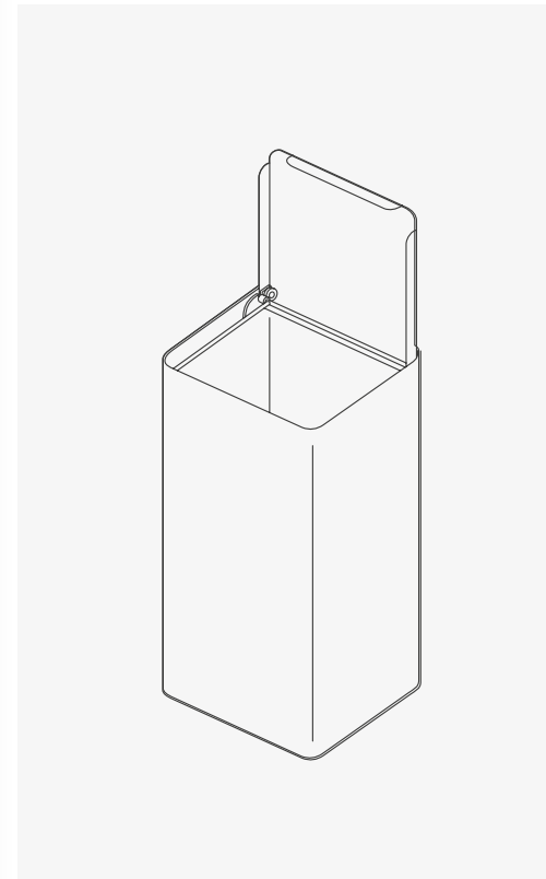
UNIX 100 cod. 1300-1301 35 x 35 – H 85 cm / 13.78" x 13.78" – H 33.46" 100 litri / 26.42 gallons – 10,0 kg / 22.05 lb
